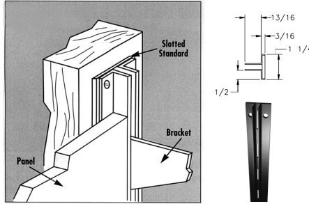
Style No. SR32
